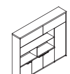
文件柜 DX90 File Cabinet W2290*D390*H1907
