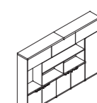
文件柜 DX92 File Cabinet W2852*D390*H1907
